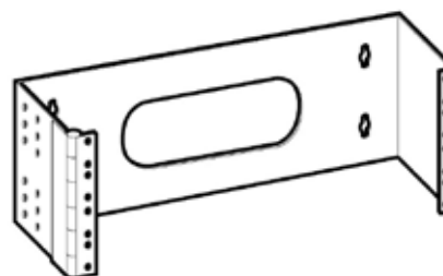
4U Shallow Wall-Mount Rack Dimensions: 178mm x 495mm x 102mm (7"H x 19.5"W x 4"D) Shipping Weight: 2.3kg (5 lb.)
