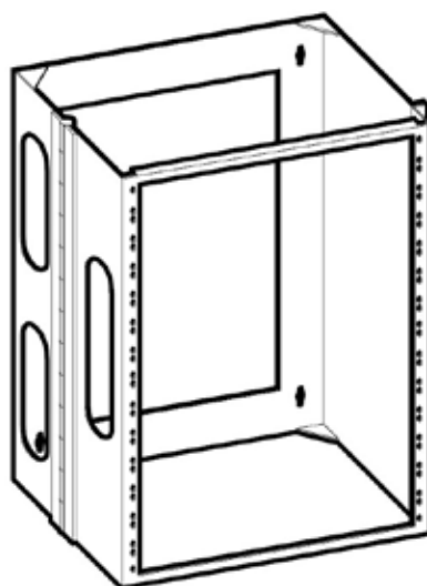
14U Deep Wall-Mount Rack Dimensions: 648mm x 489mm x 203mm (25.5"H x 19.25"W x 8"D) Shipping Weight: 12.7kg (28 lb.)
