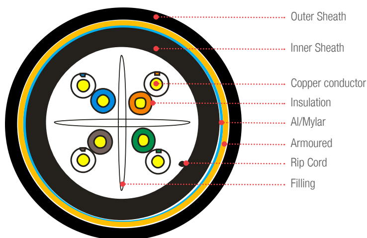
PowerCat™ 6 U/UTP Outdoor Cable
