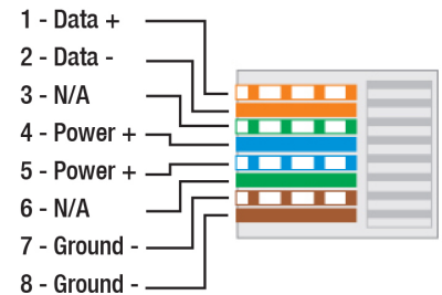
CoreSync Cable Pinout (RJ45 connector)
