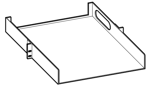
2U Equipment Shelf Dimensions: 89mm x 483mm x 406mm (3.5"H x 19"W x 16"D) Shipping Weight: 2kg (4 lb. 6oz.)
